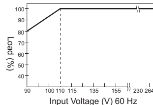
Figure 5 Relation between output power and input voltage
