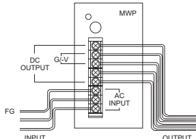
Figure 2 Wiring and connection
