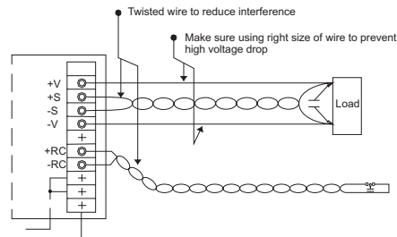
Figure 6 Remote ON/OFF and sensing wiring
