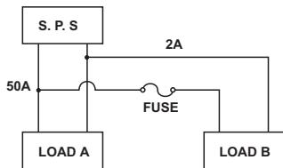
Figure 12: Output wiring
