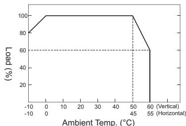
Figure 4 Relation between output power and temperature (derating curve)
