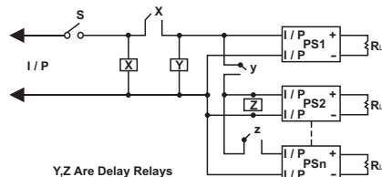
Figure 13: Delay circuit
