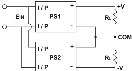
Figure 10: Positive and negative terminals connect in series
