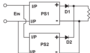
Figure 8: Paralleling with adding diodes in series connection
