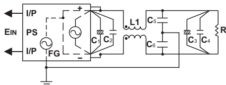
Figure 15: Ripple noise suppression
