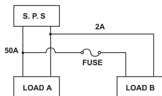
Figure 12: Output wiring
